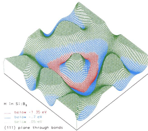
FIG. 1. Energy surface for an H atom in the (111) plane through three bond-minima ( BM ) positions in Si:B 5 . The plane does not contain atoms, but the unrelaxed lattice position of the B atom is located just 0.4 Å outside the plane in the center of the red ring. The contours are color coded in three different ranges for presentation purposes. For clarity, the surface is cut off at an energy value of 0.05 eV, resulting in the green plateaus. The zero of energy is chosen at the tetrahedral interstitial site.
