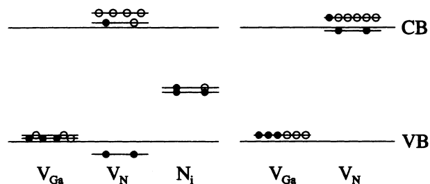
FIG. 2. Schematic representation of the location of defect levels for the gallium and nitrogen vacancies, and the nitrogen split interstitial. The results of a tight-binding calculation by Jenkins and Dow (Ref. 6) are shown on the right. The occupations are shown for the neutral charge state; filled circles indicate electrons, open circles indicate holes.
