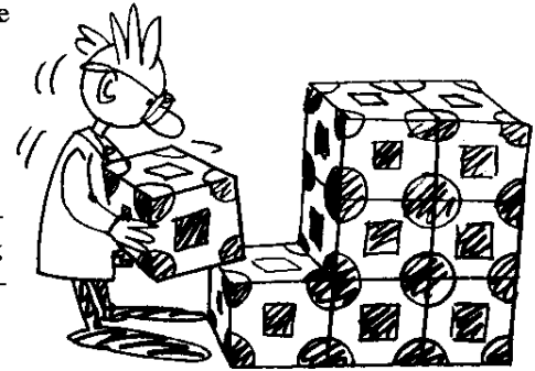
unit cell
