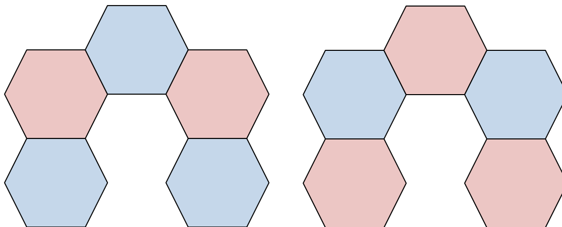
Corannulene "caps"
