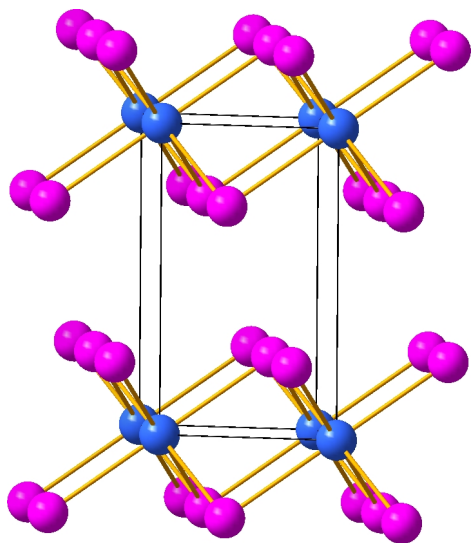
\text{CdI}_2
