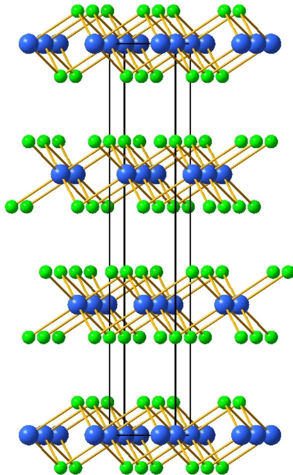
\text{CdCl}_2
