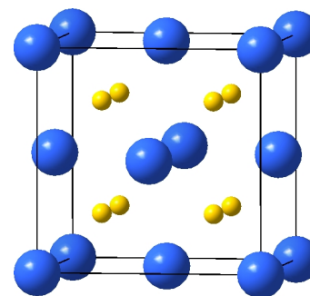
\text{CaF}_2
