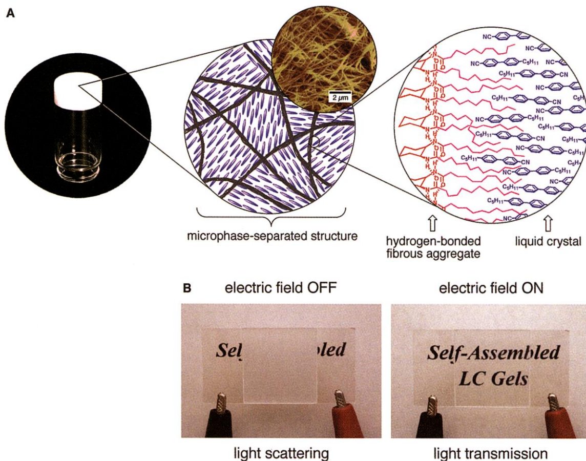
Fig. 4. Micrometer-scale phase segregation of liquid-crystalline physical gels. (A) Hierarchical structures consisting of self-assembled fibers and conventional rodlike liquid crystals. (B) Left, light-scattering state (with the electric field off); right, light-transmission state (with the electric field on).
