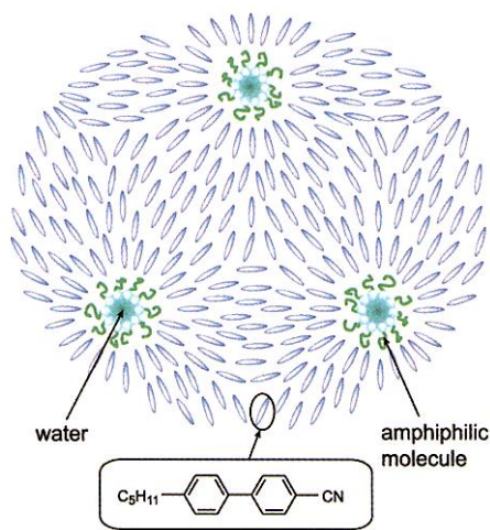
Fig. 5. Nanometer-scale 3D phase segregation of inverse micelles and conventional rodlike liquid crystals. A transparent nematic phase is shown.
