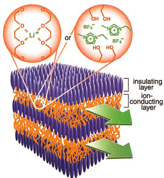
Fig. 3. Nanometer-scale 2D phase-segregation in smectic phases consisting of lithium salts and rod-coil-rod molecules containing PEO moieties or conventional ionic liquids and hydroxyl-terminated rodlike molecules.
