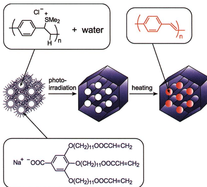
Fig. 2. Nanometer-scale 1D phase segregation. Self-assembly and fixation of a hexagonal columnar phase containing a conductive polymer are shown.
