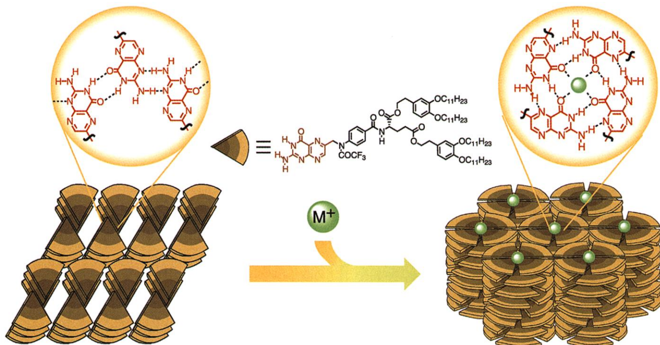
Fig. 1. Ion-responsive self-assembled liquid crystals. Ribbonlike structures of a folic acid derivative and their structural change to the disklike tetramers by the addition of metal ions ( M^+ ) are shown.
